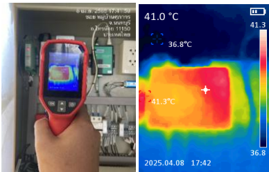
Switch Hub 41.0 °C
